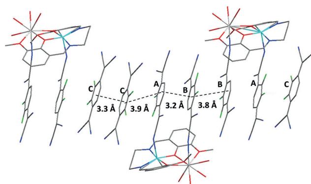
Figure 2. Side view of the quasi-1D chain showing the distances between adjacent TCNQF species (ring centroids) in the structure of compound 1 (A–B: 3.210(1) Å, B–B: 3.761(2) Å, A–C: 3.885(2) Å, C–C: 3.266(1) Å). Fluorine atoms are disordered in two positions on each of the TCNQF radicals.
